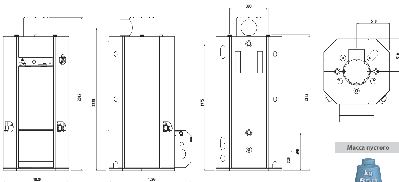
HeatMaster® 201
