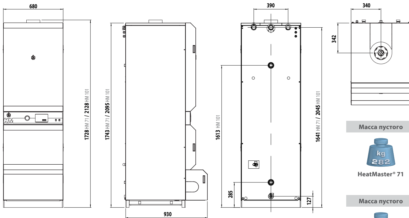
HeatMaster® 71 / 101
